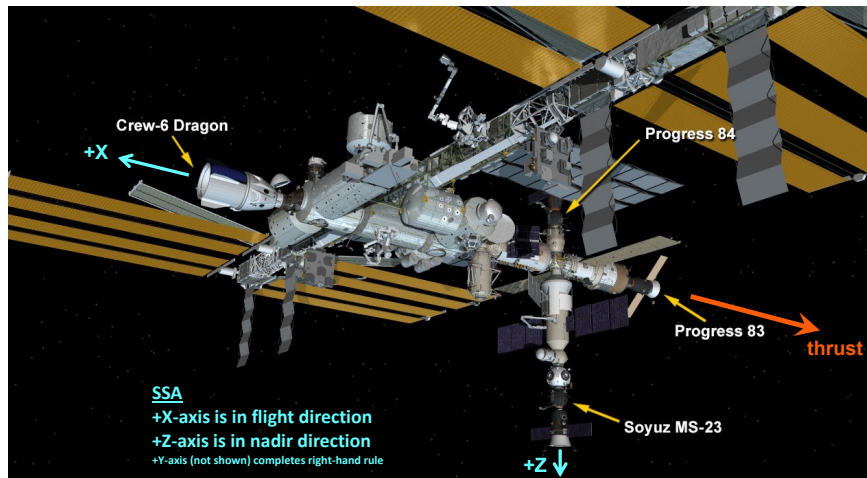
Fig. 1: Progress 83P's Location and Alignment during Reboost.
