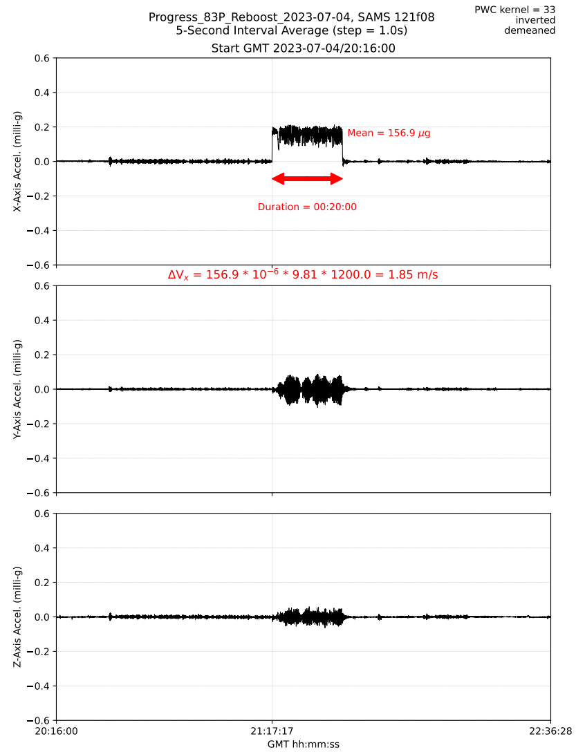
Fig. 9: 5-sec interval average for SAMS 121f08 sensor in the COL.
