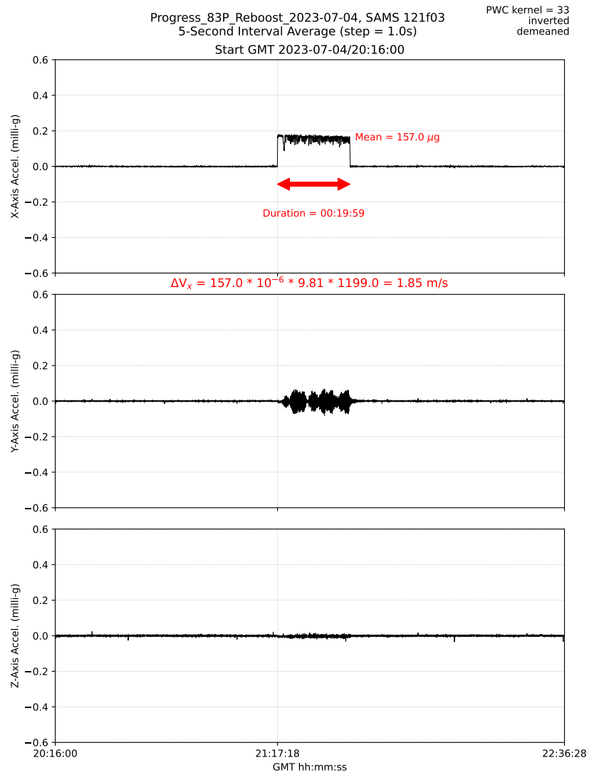
Fig. 4: 5-sec interval average for SAMS 121f03 sensor in the LAB.
