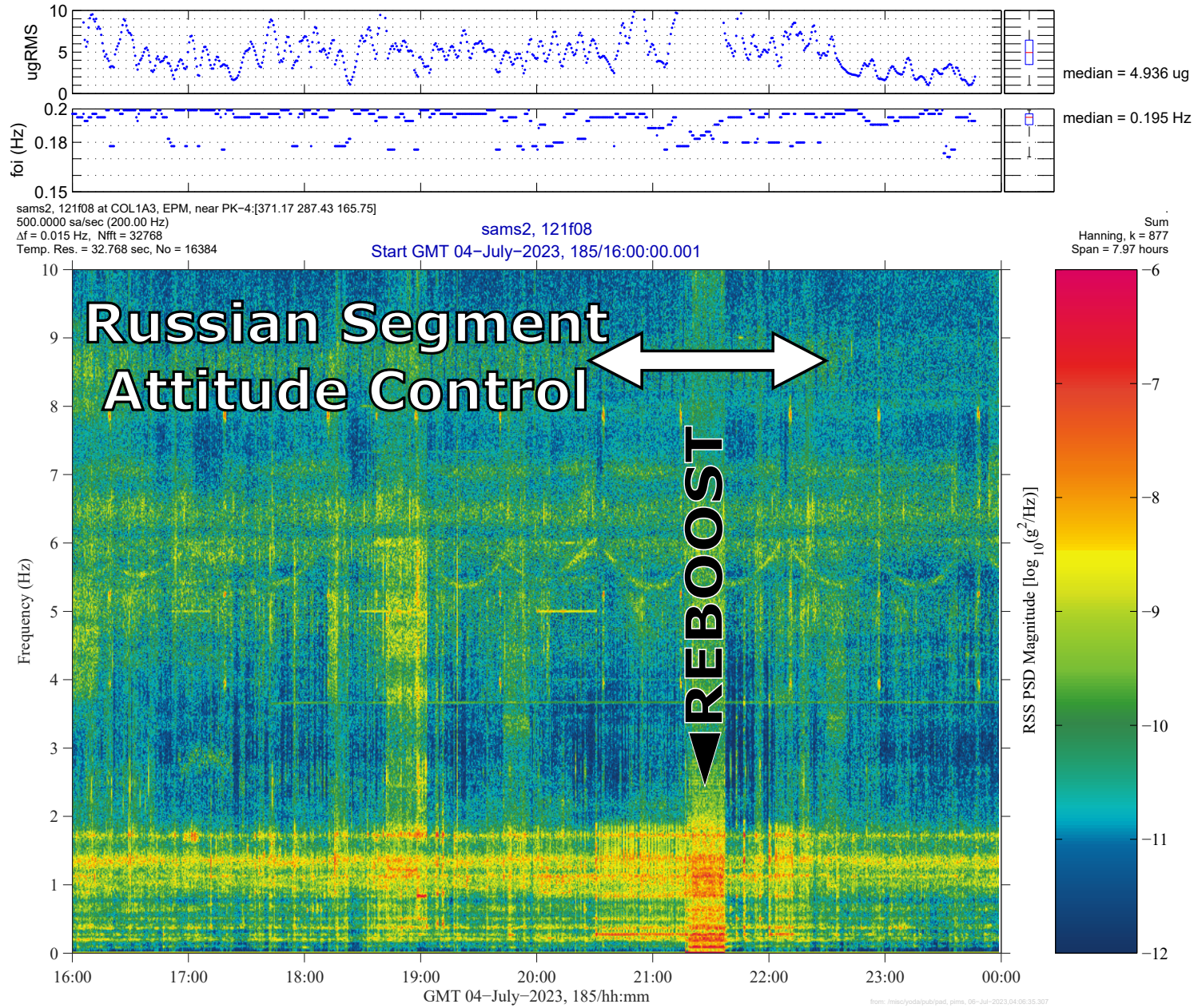
Fig. 2: 10 Hz Spectrogram showing Progress 83P Reboost on GMT 2023-07-04 from a SAMS Sensor in Columbus Module.
