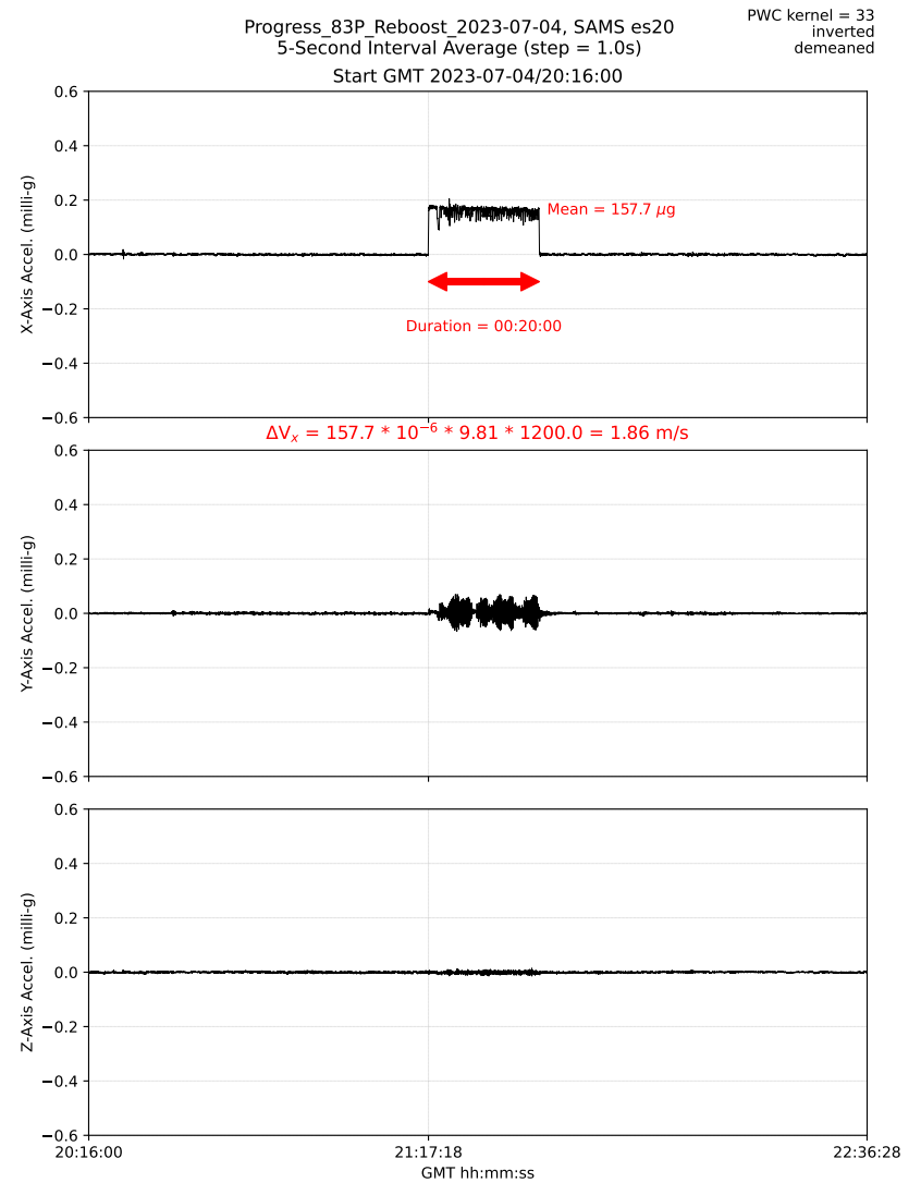
Fig. 7: 5-sec interval average for SAMS es20 sensor in the LAB.
