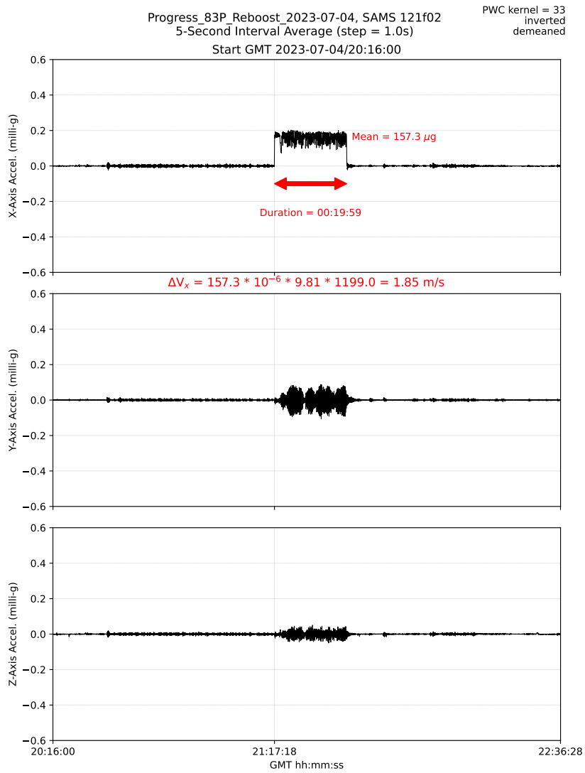
Fig. 8: 5-sec interval average for SAMS 121f02 sensor in the COL.
