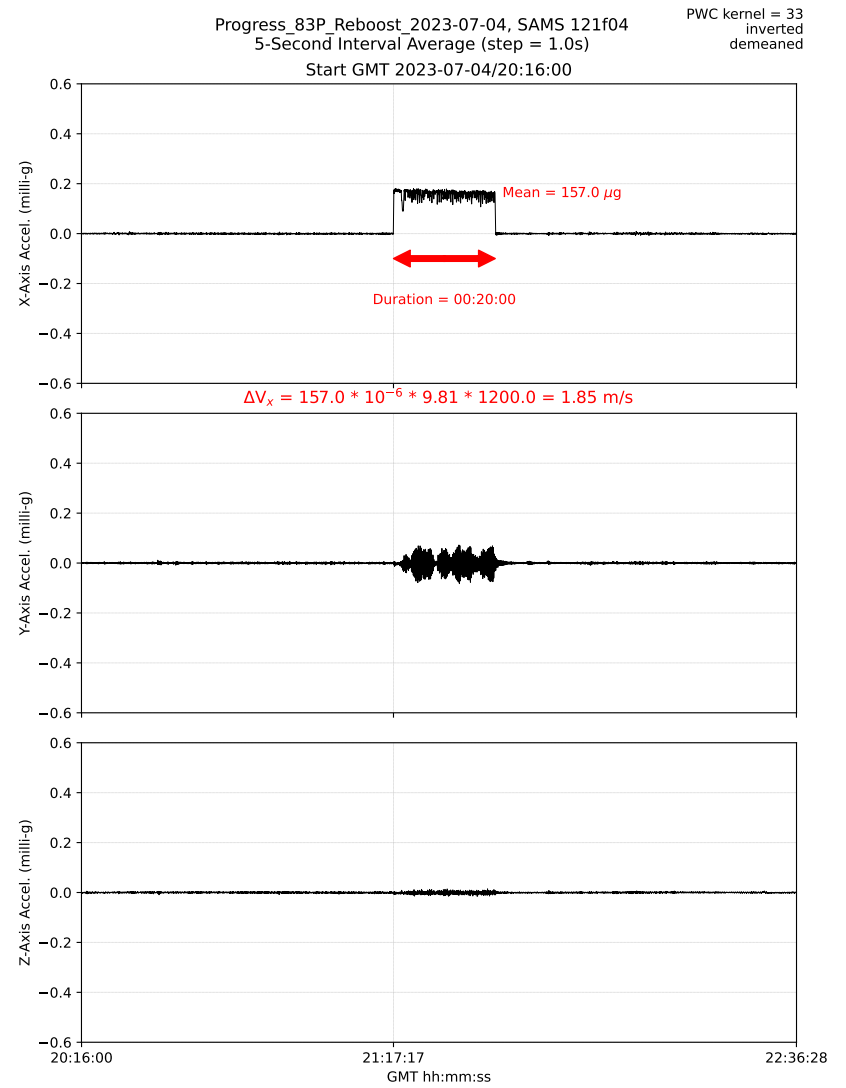
Fig. 5: 5-sec interval average for SAMS 121f04 sensor in the LAB.
