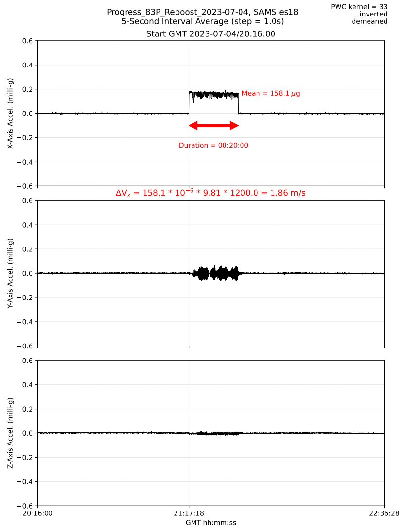
Fig. 6: 5-sec interval average for SAMS es18 sensor in the LAB.
