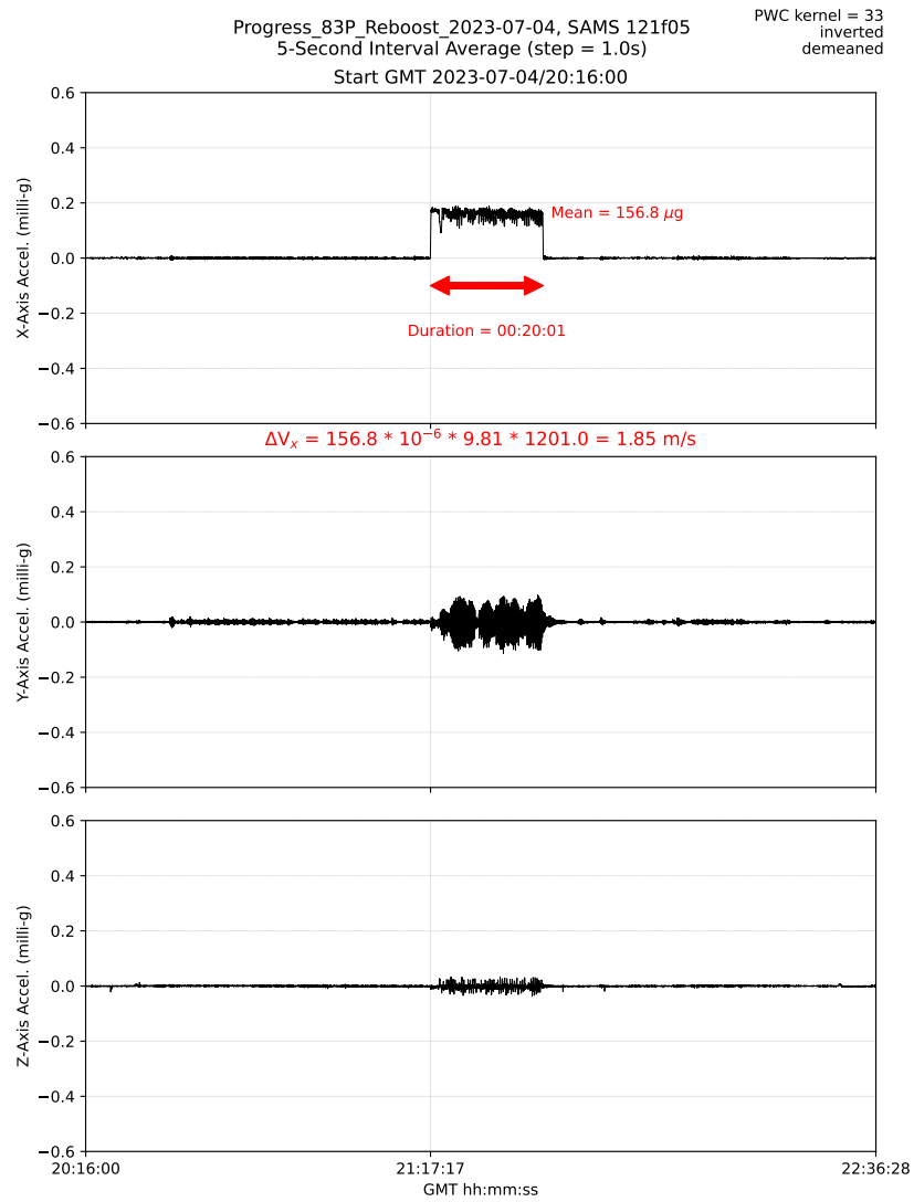
Fig. 10: 5-sec interval average for SAMS 121f05 sensor in the JEM.
