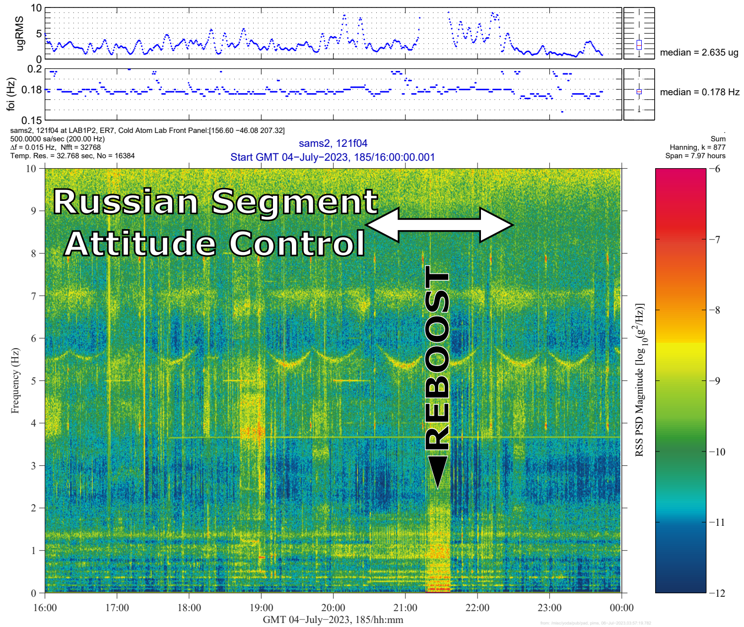
Fig. 3: 10 Hz Spectrogram showing Progress 83P Reboost on GMT 2023-07-04 from a SAMS Sensor near Cold Atom Lab in US Lab.
